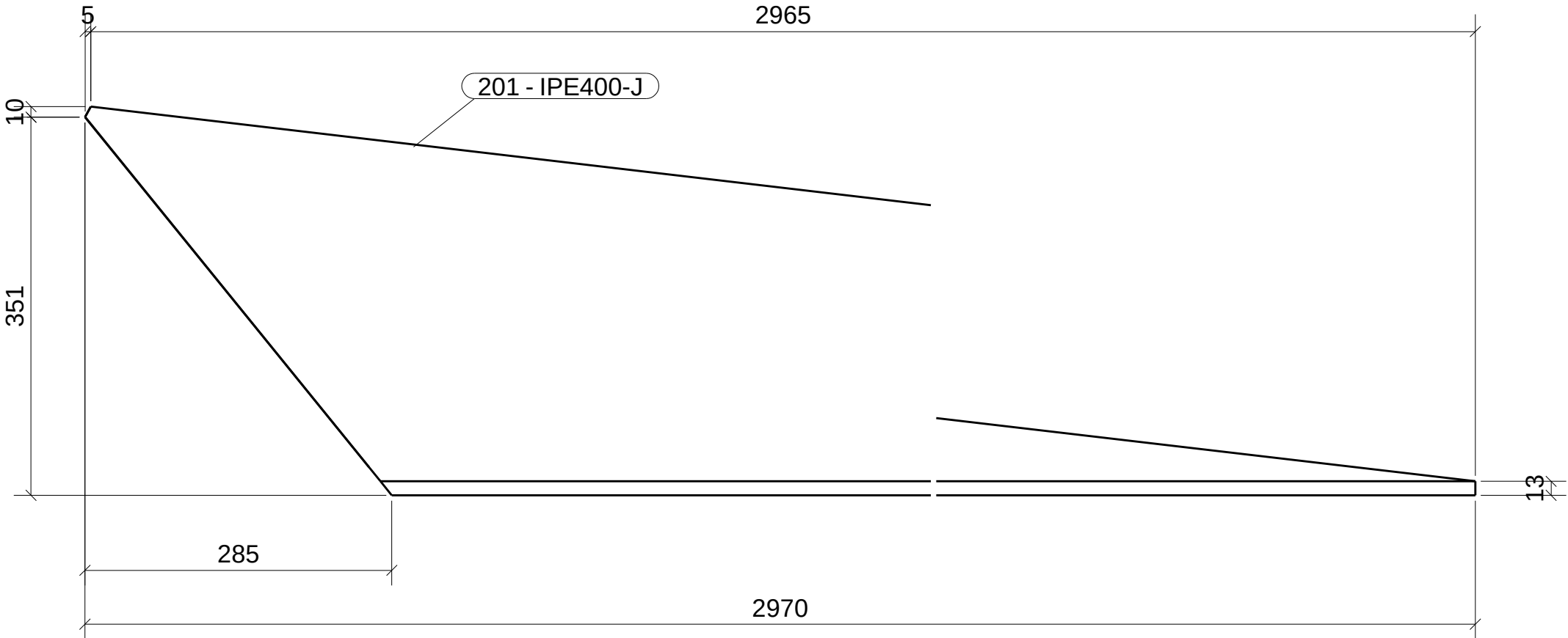
FRONT VIEW
